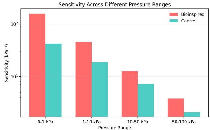
Figure 11. Sensitivity Across Different Pressure Ranges. The bioinspired sensor consistently outperforms the control sensor across all pressure ranges, with a logarithmic decrease in sensitivity that mimics human tactile perception.
