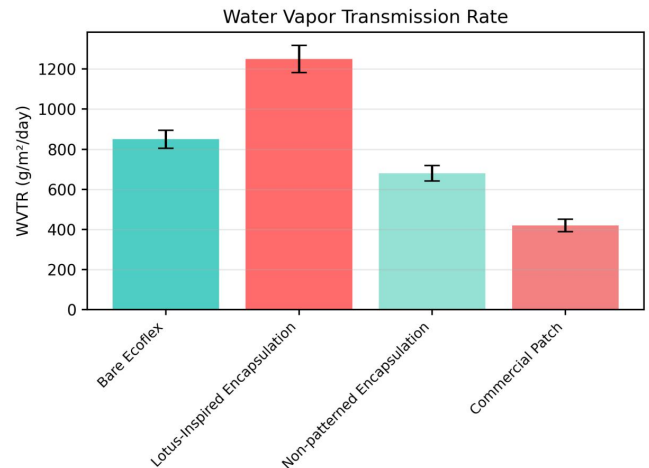
Figure 9. Water Vapor Transmission Rate. The bioinspired encapsulation layer shows a significantly higher WVTR compared to non-patterned materials and commercial patches, indicating superior breathability.
